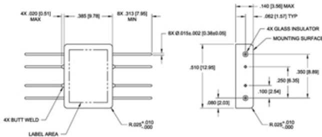
Weight: 0.0568 ± oz w/o connectors and spacer plate, ± 0.004 oz
